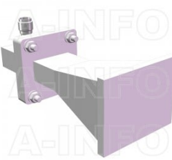
LB-112-10-C-TFSPO Standard Gain Horn Antenna 7.05-10GHz 10dB Gain TNC Female
