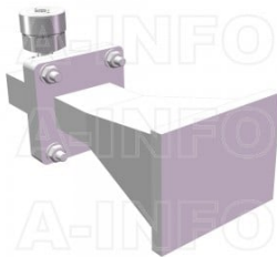
LB-112-10-C-7SPO Standard Gain Horn Antenna 7.05-10GHz 10dB Gain 7mm Female
