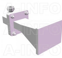
LB-112-10-C-NFSPO Standard Gain Horn Antenna 7.05-10GHz 10dB Gain N Type Female
